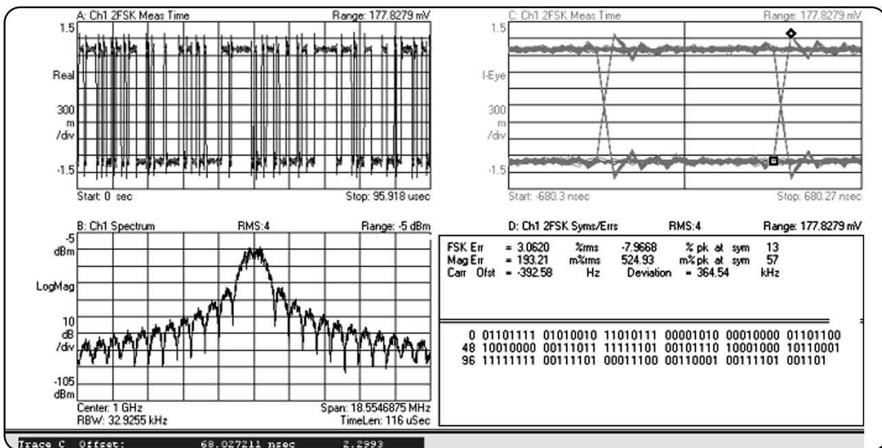
Figure 1.1.1: 2-FSK signal characteristics
