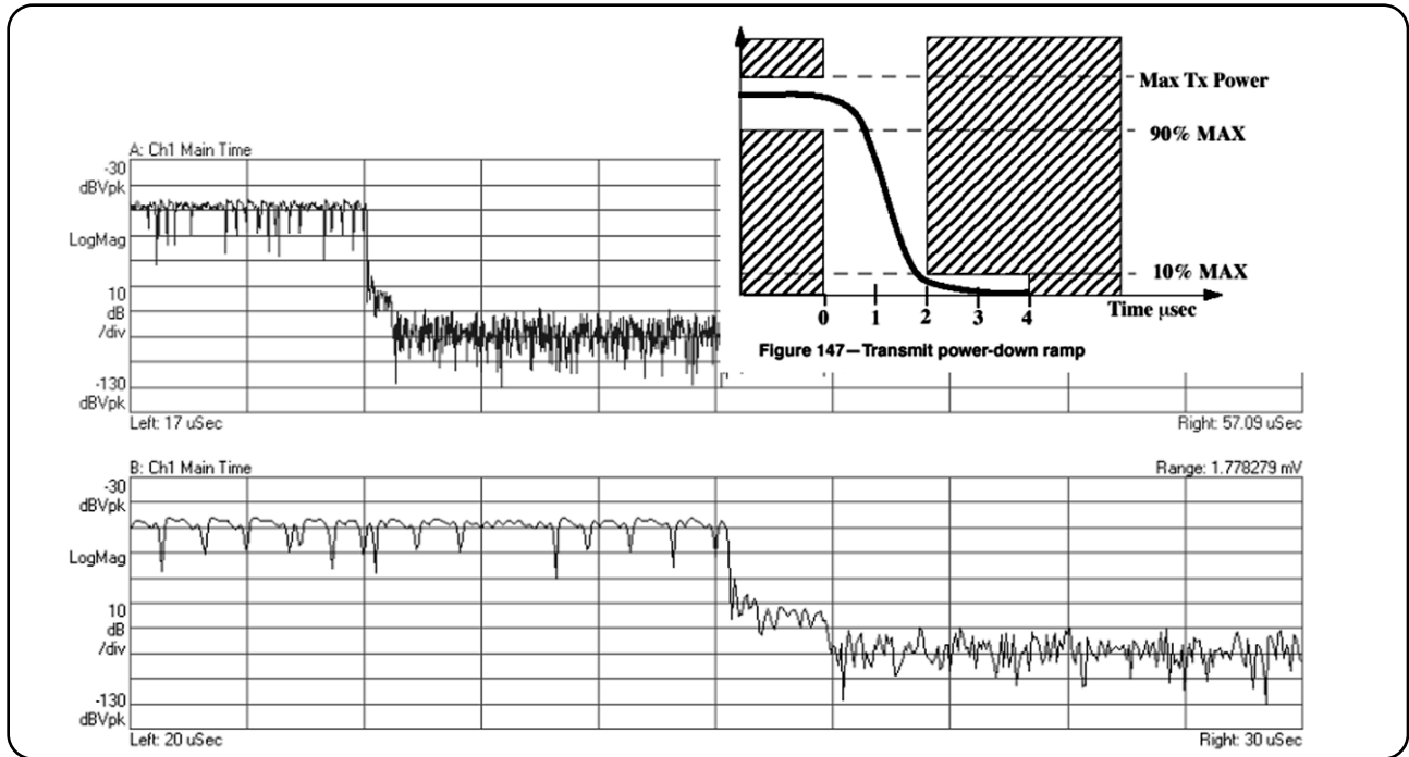
Figure 2.3.6: 802.11b power-down-envelope mask
