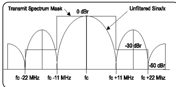
Figure 2.3.7: 802.11b transmit spectral mask
